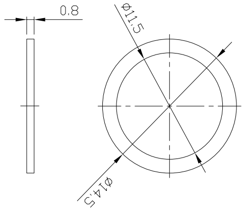
WASHER
