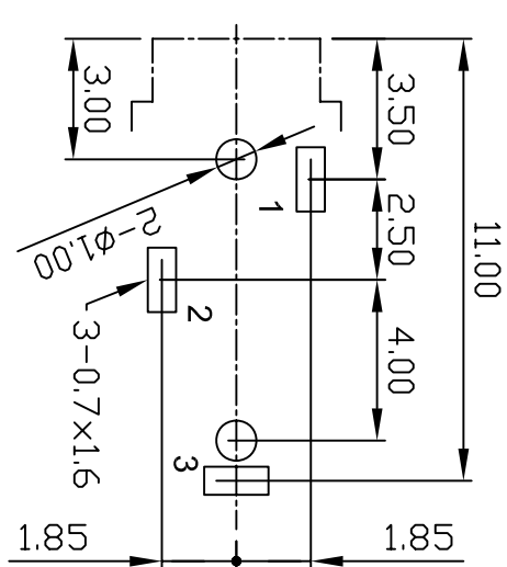
PCB LAYOUT(±0.1) (BOTTOM VIEW)
