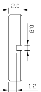
P.C.B LAYOUT (±0.1) (BOTTOM VIEW)
