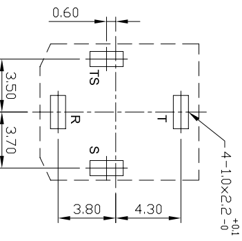
P.C.B LAYOUT (±0.1) (BOTTOM VIEW)
