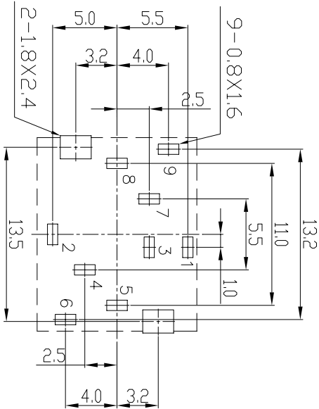
P.C.B. LAYOUT(tol±0.1) (BOTTOM VIEW)
