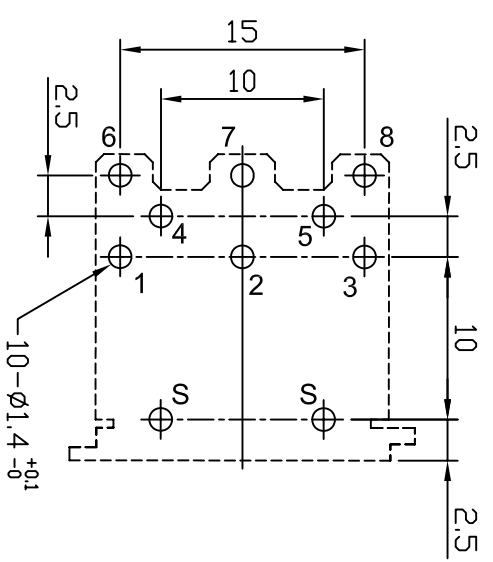
P.C.B LAYOUT( \pm 0.1 ) (BOTTOM VIEW)
