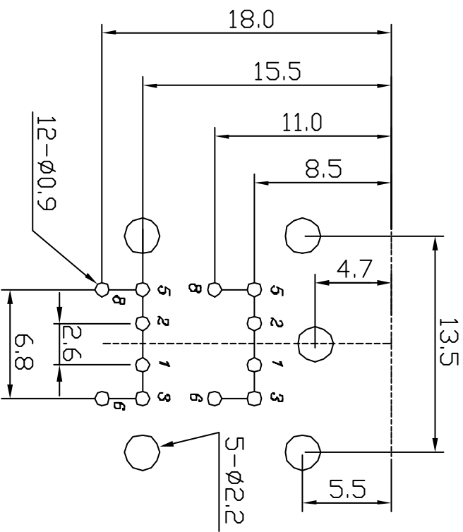
P.C.B LAYOUT( \pm 0.1 ) (BOTTOM VIEW)
