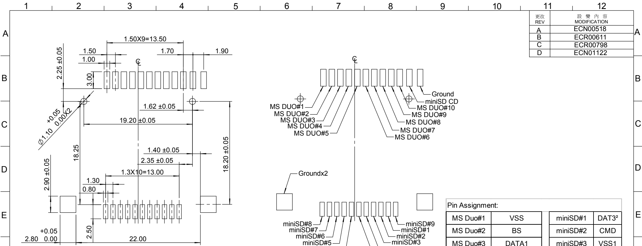
PCB Layout for Modile Phone MP3 Camera Single Slot Card Reader
