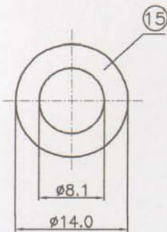
WASHER t=0.4
