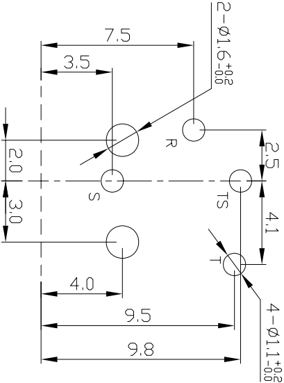
P.C.B. LAYOUT(±0.1) (BOTTOM VIEW)
