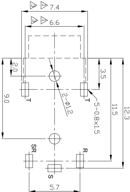
P.C.B LAYOUT (BOTTOM VIEW)
