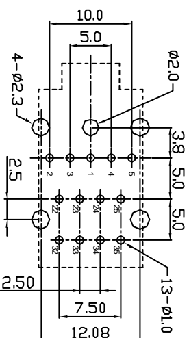
PCB LAYOUT(±0.1) BOTTOM VIEW
