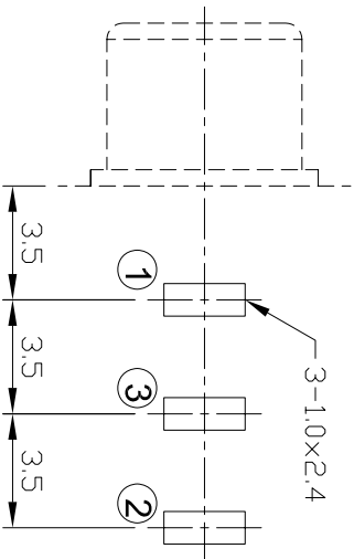
PCB LAYOUT (BOTTOM VIEW) \Delta
